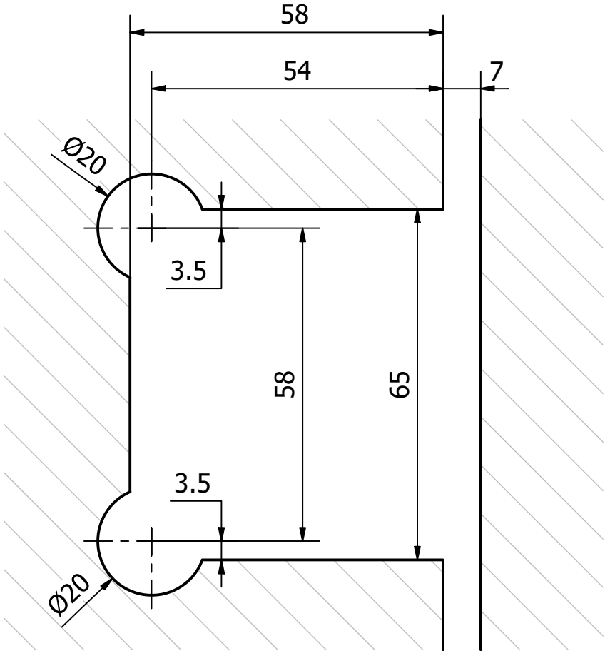
530 Glass to wall cutout 10 -12 mm glass
